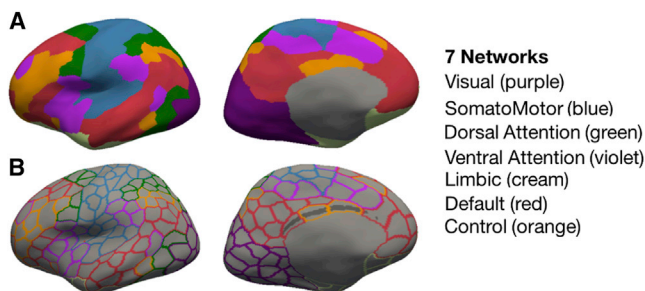
Figure 2. Parcellation Scheme
